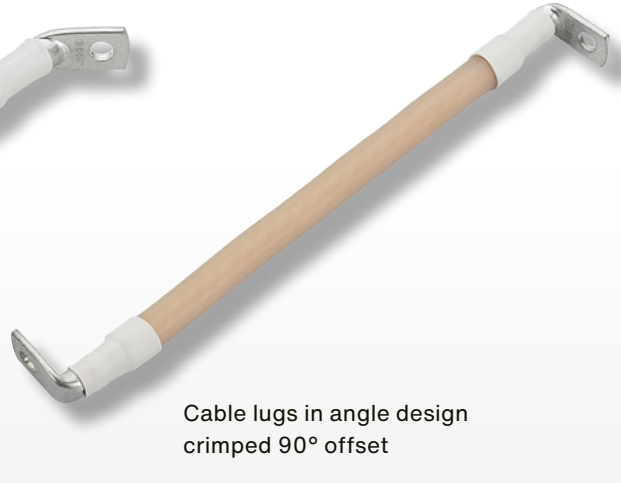
Cable lugs/Angle design 45° or 90°
