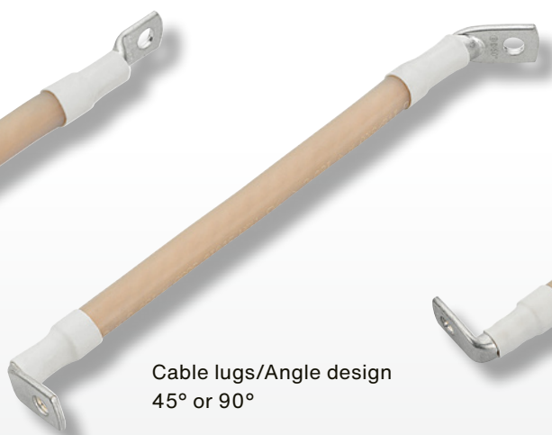
Cable lugs in angle design crimped 90° offset
