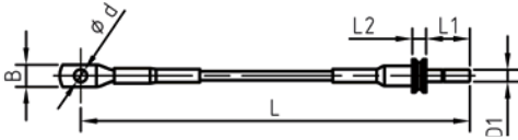
Design A with plug
